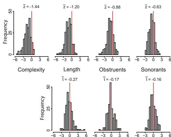
Fig. 3. (Upper) Histograms of z -transformed rank-order correlations between an attribute score and word frequency for four attributes related to ease of pronunciation: complexity, length, obstruents, and sonorants ( n = 232 meanings; SI Appendix ). All z scores, P < 1^{-10} . (Lower) Histograms of t scores after controlling for complexity (responses with more words have more sounds). Length remains significant ( P < 0.002 ), while effect sizes are small (average t = -0.21 ) for obstruents ( P = 0.06 ) and sonorants ( P = 0.04 ). Controlling for length, the effect of obstruents and sonorants disappears ( P > 0.35 ).
